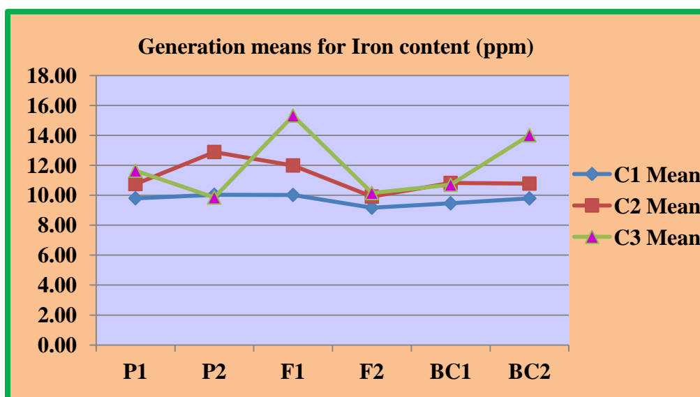
Fig. 1. Mean values of 6 Generations of 3 crosses for Iron content
