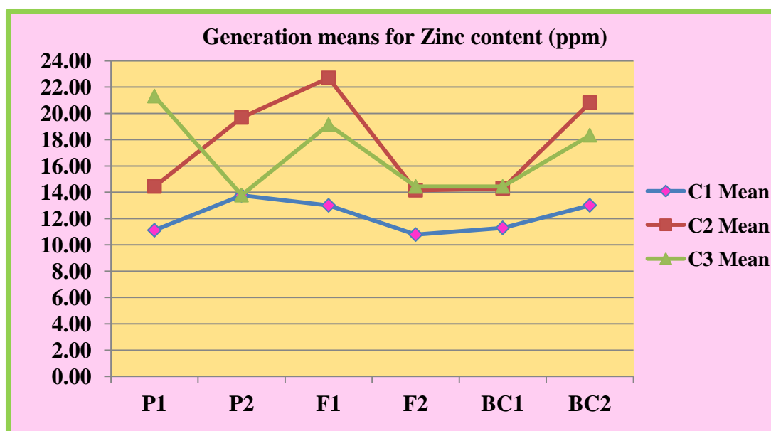
Fig. 2. Mean values of 6 generations of 3 crosses for zinc content
