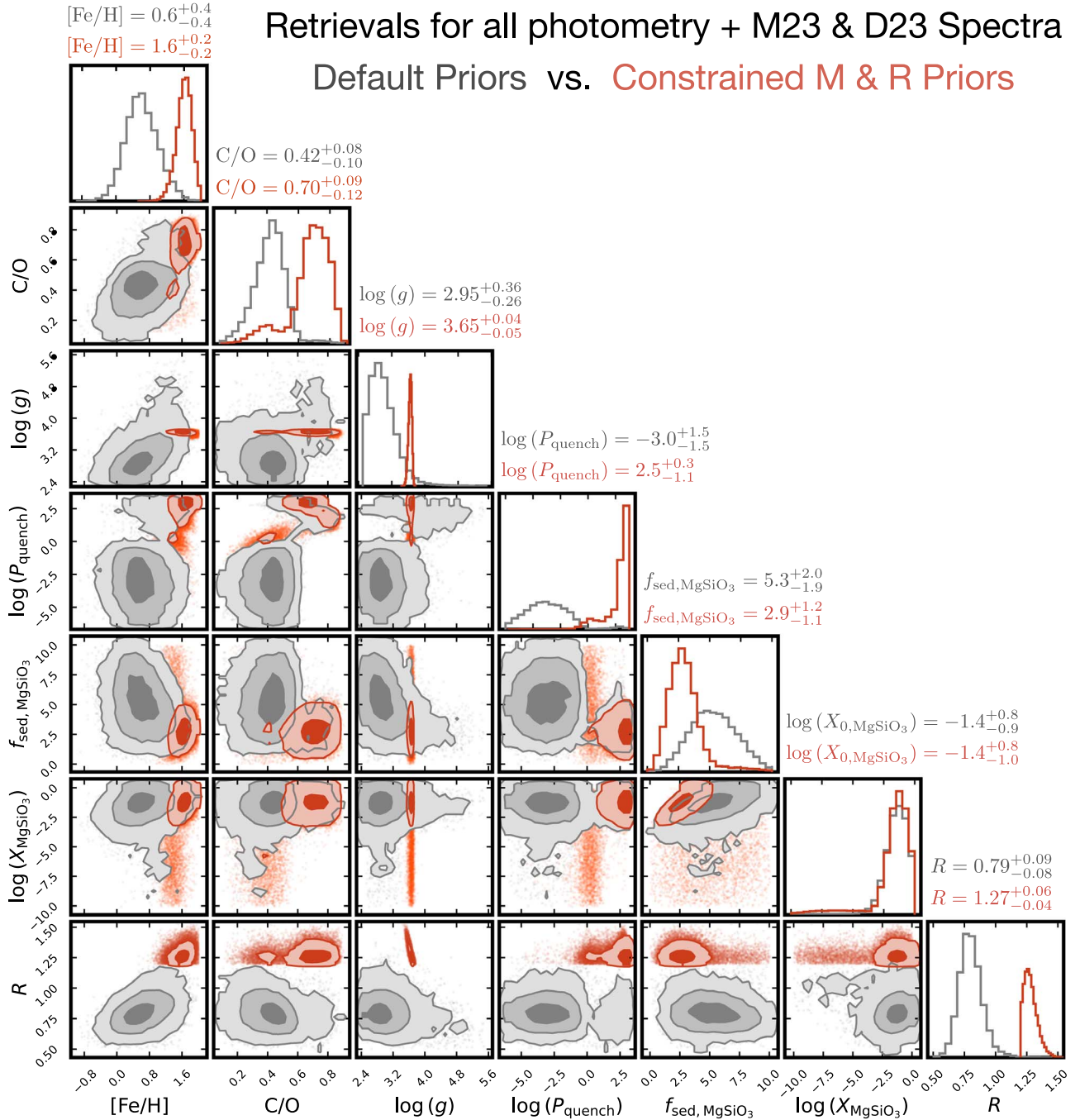
Figure 10. Corner plot for the retrieval runs performed with default parameter priors (gray) and with constrained priors on the planet’s mass, \mathcal{N}(\mu = 2.8 M_{\text{Jup}}, \sigma = 0.6 M_{\text{Jup}}) , and radius, \mathcal{U}(1.20 R_{\text{Jup}}, 1.55 R_{\text{Jup}}) (orange). We show 1\sigma/2\sigma/3\sigma confidence intervals for parameters inferred by the former retrieval (with default priors), but only present 1\sigma/2\sigma confidence intervals for the latter in order to prevent visual overlap. Both retrieval runs are performed on K1/K2/L' photometry and both the Mesa et al. (2023) and De Rosa et al. (2023) spectra (Section 7.3).
