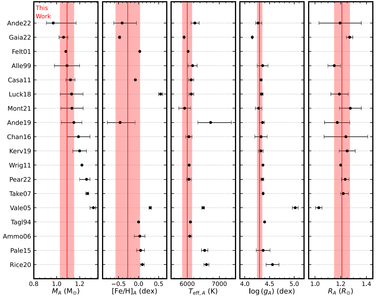
Figure 16. Our measured stellar parameters of AF Lep A (vertical red line with shadow) compared to those in the literature (black; sorted by M_A , and then by [\text{Fe}/\text{H}]_A if M_A is not reported). References for labels shown on the y-axis are as follows. Tagl94: Tagliaferri et al. (1994); Alle99: Allende Prieto & Lambert (1999); Felt01: Feltzing et al. (2001); Vale05: Valenti & Fischer (2005); Ammo06: Ammons et al. (2006); Take07: Takeda et al. (2007); Casa11: Casagrande et al. (2011); Wrig11: Wright et al. (2011); Pale15: Paletou et al. (2015); Chan16: Chandler et al. (2016); Luck18: Luck (2018); Ande19: Anders et al. (2019); Kerv19: Kervella et al. (2019); Rice20: Rice & Brewer (2020); Mont21: Montalto et al. (2021); Ande22: Anders et al. (2022); Gaia22: Gaia Collaboration et al. (2023); Pear22: Pearce et al. (2022).
