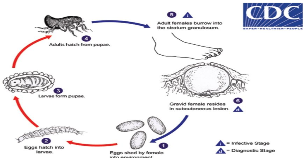
Fig. 2. Diagram showing the life cycle of Tunga penetrans
