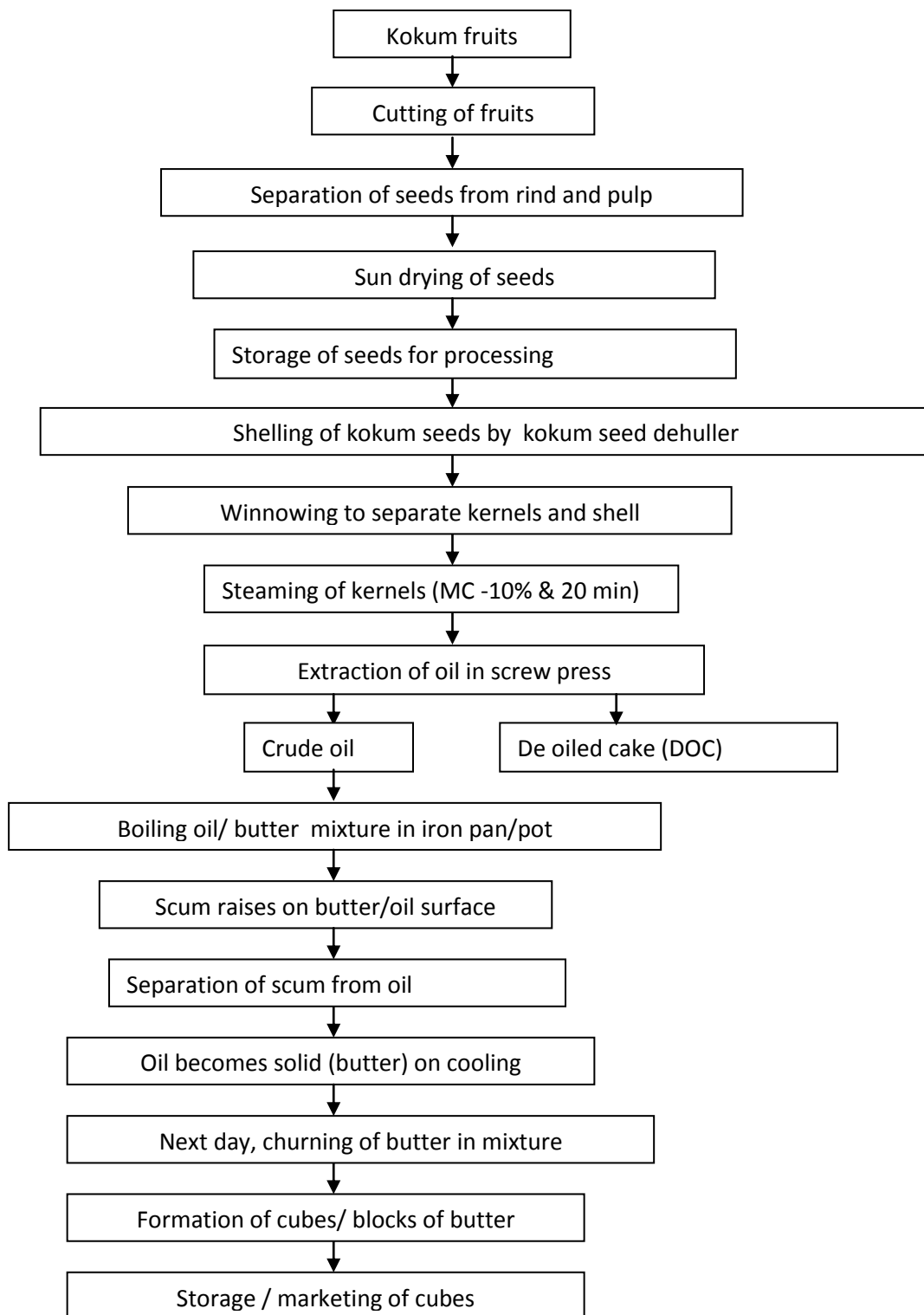
Fig. 1. Flow chart for Standardization of Kokum Butter extraction
