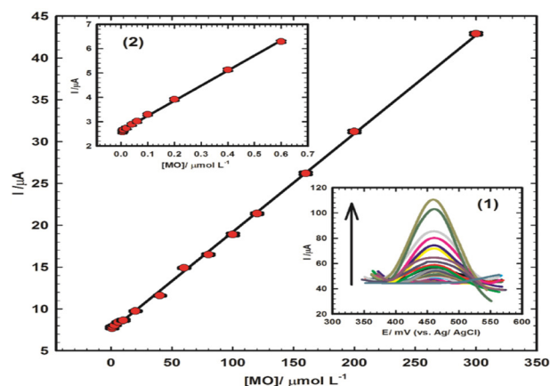
Figure 5. Calibration curve for morphine (MO) in the linear range (0.8 μmol L -1 – 300 μmol L -1 ) at CoGILCCP-SDS. Inset (1): Differential pulse voltammograms (DPVs) of MO in urine at CoGILCCP-SDS for concentrations from (5 nmol L -1 to 300 μmol L -1 ). Inset (2): Calibration curve for MO in the linear range (5 nmol L -1 – 0.6 μmol L -1 ) at CoGILCCP-SDS.
