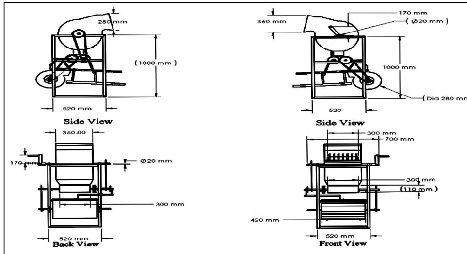
Fig. 1. Overall dimension of manually operated modified linseed crop thresher
