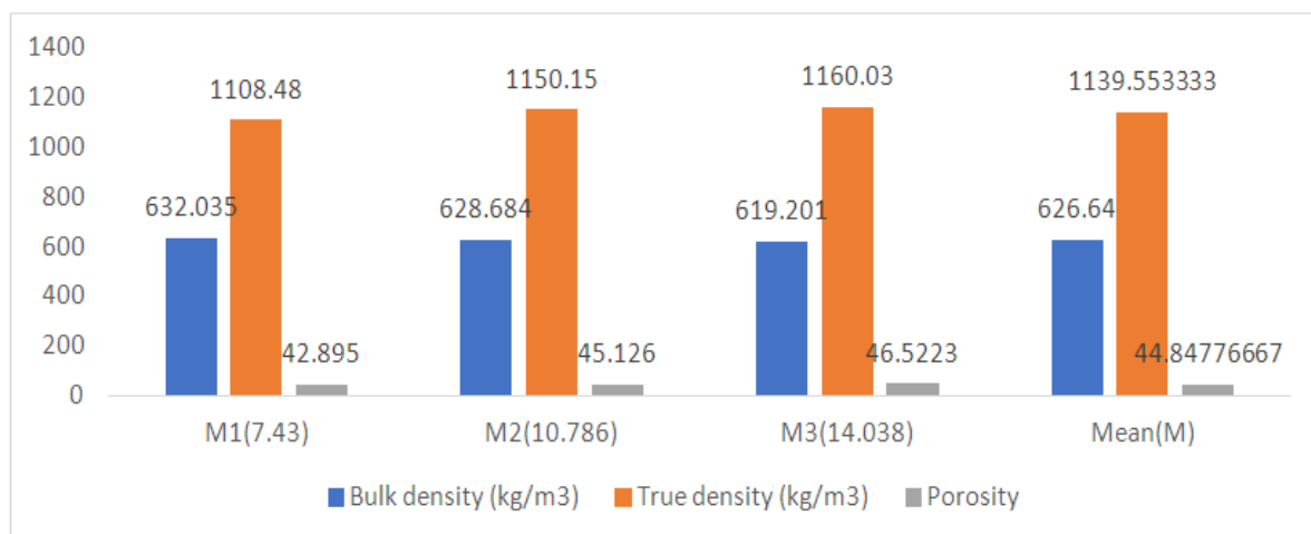
Fig. 7. Moisture content's effect on bulk density, true density and porosity of linseed variety in SHUATS Alsi-2
