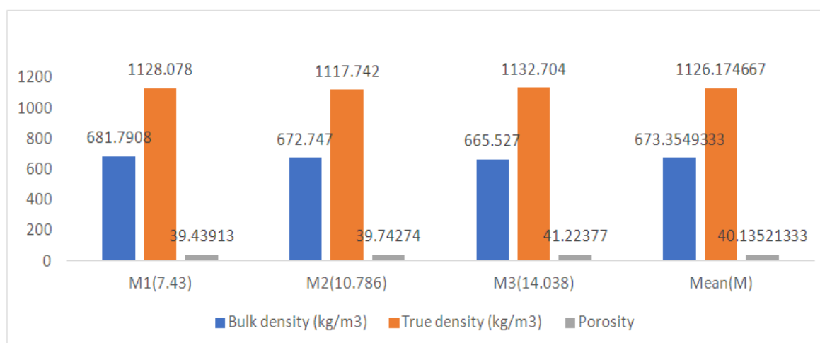
Fig. 8. Moisture content's effect on bulk density, true density and porosity of linseed variety in Neelam
