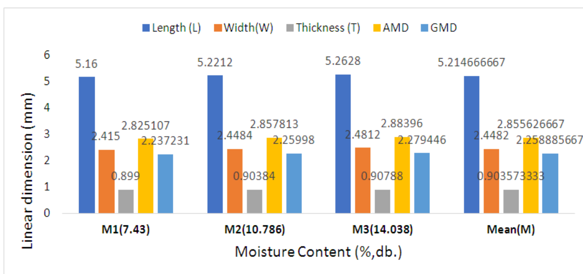
Fig. 4. Moisture content's effect on linear dimensions of linseed variety in Neelam
