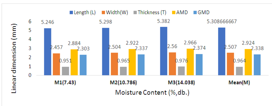
Fig. 3. Moisture content's effect on linear dimensions of linseed variety in SHUATS Alsi-2
