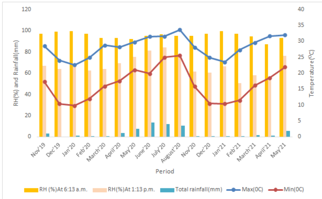
Fig. 1. Metereological data observed during the experimental periods (2020-2021)
