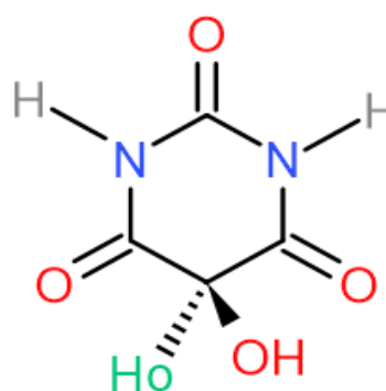
Fig. 2. Chemical structure of Alloxan
