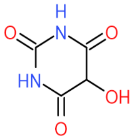
Fig. 3. Structure of Dialuric acid i.e reduction product of alloxan
