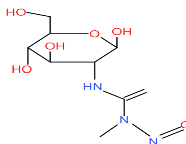
Fig. 1. Chemical structure of streptozocin
