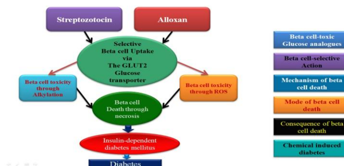
Fig. 4. A visual representation of streptozotocin and alloxan's damaging effects on beta cells
