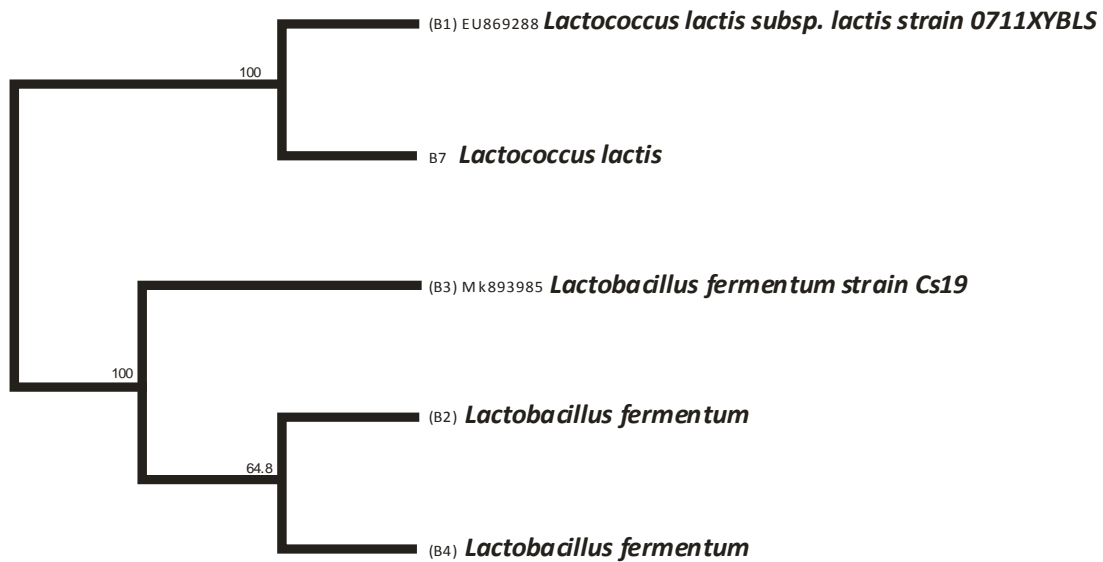
Fig. 2. Phylogenetic tree showing the evolutionary distance between the bacterial isolates
