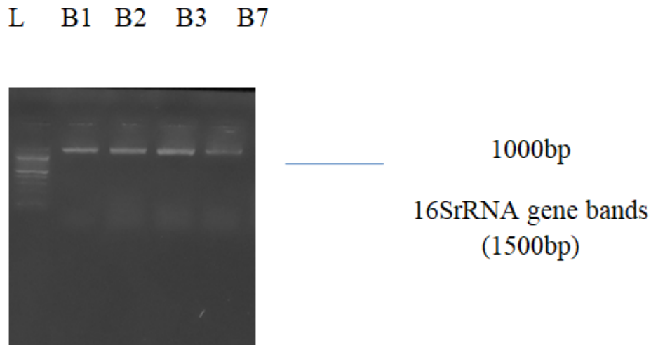
Fig. 1. Agarose gel electrophoresis of the 16SrRNA gene of some selected bacterial isolates. Lanes B1-B7 represent the 16SrRNA gene bands (1500bp), Lane L represents the 100bp molecular ladder
