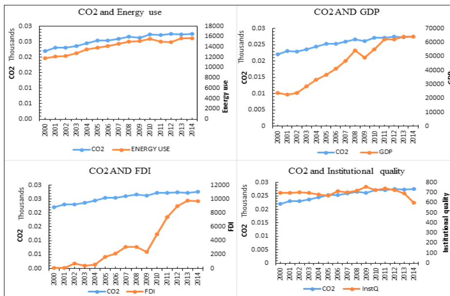
Fig. 2. Energy use, GDP, FDI, Institutional quality and carbon emission nexus
