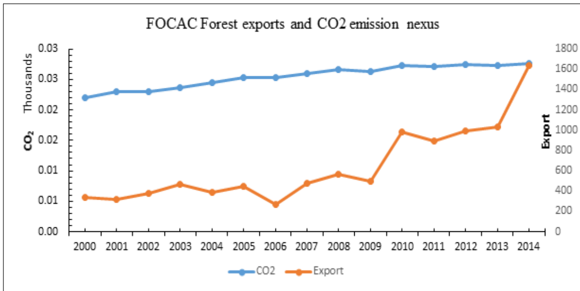
Fig. 1. Forest export and carbon emissions
