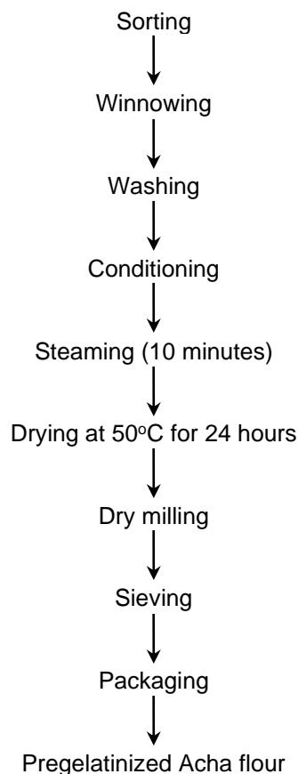
Fig. 1. Flow chart for the production of Pregelatinized Acha Flour (PAF) [21]
