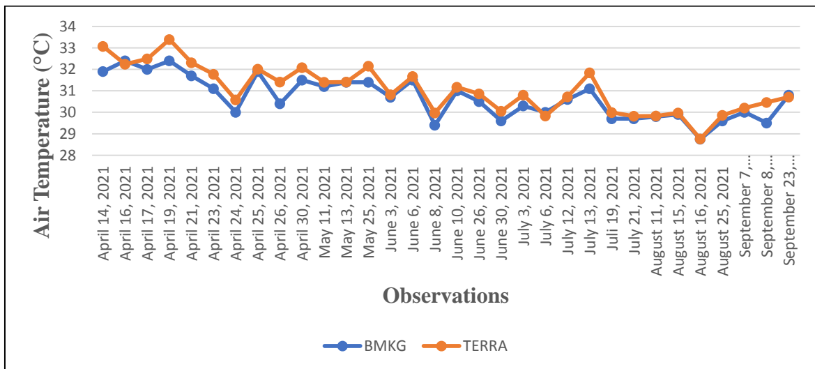
Fig. 5. Terra MODIS air temperature pattern with BMKG air temperature
