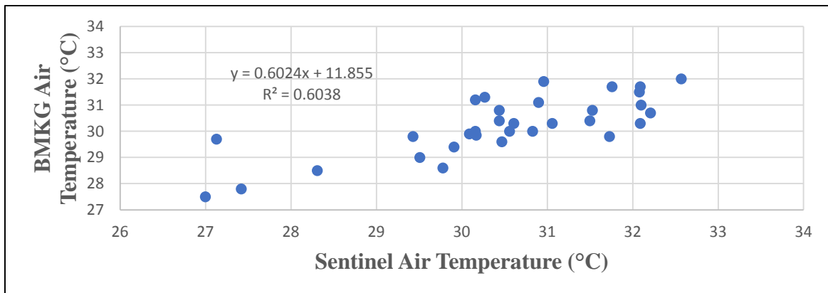
Fig. 4. Scatter plot of Sentinel-3 air temperature with BMKG air temperature
