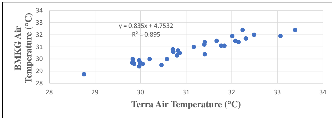
Fig. 6. Scatter plot of terra MODIS air temperature with BMKG air temperature
