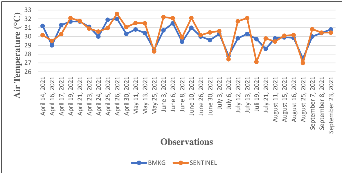
Fig. 3. Sentinel-3 air temperature pattern with BMKG air temperature
