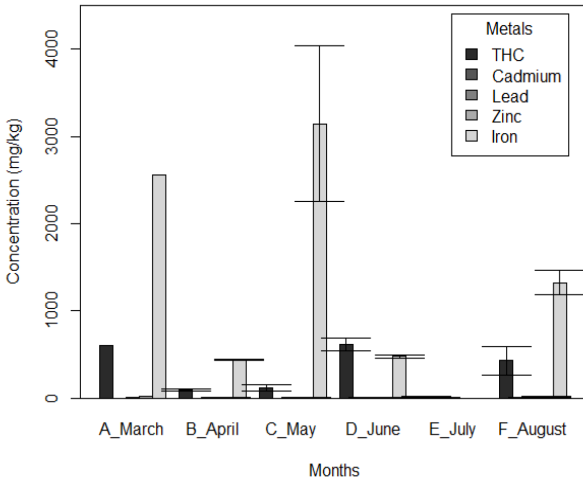
Fig. 5. Mean monthly heavy metal concentration (±SE) of nypa palm ( Nypa fruticans ) parts treated soil
