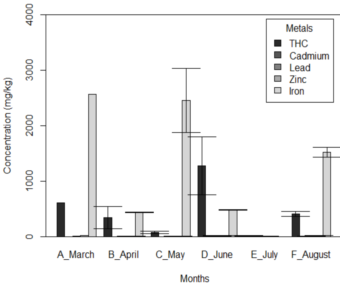
Fig. 6. Mean monthly THC and heavy metal concentration ( \pm SE) of mangrove ( Rhizophora racemosa ) treated soil
