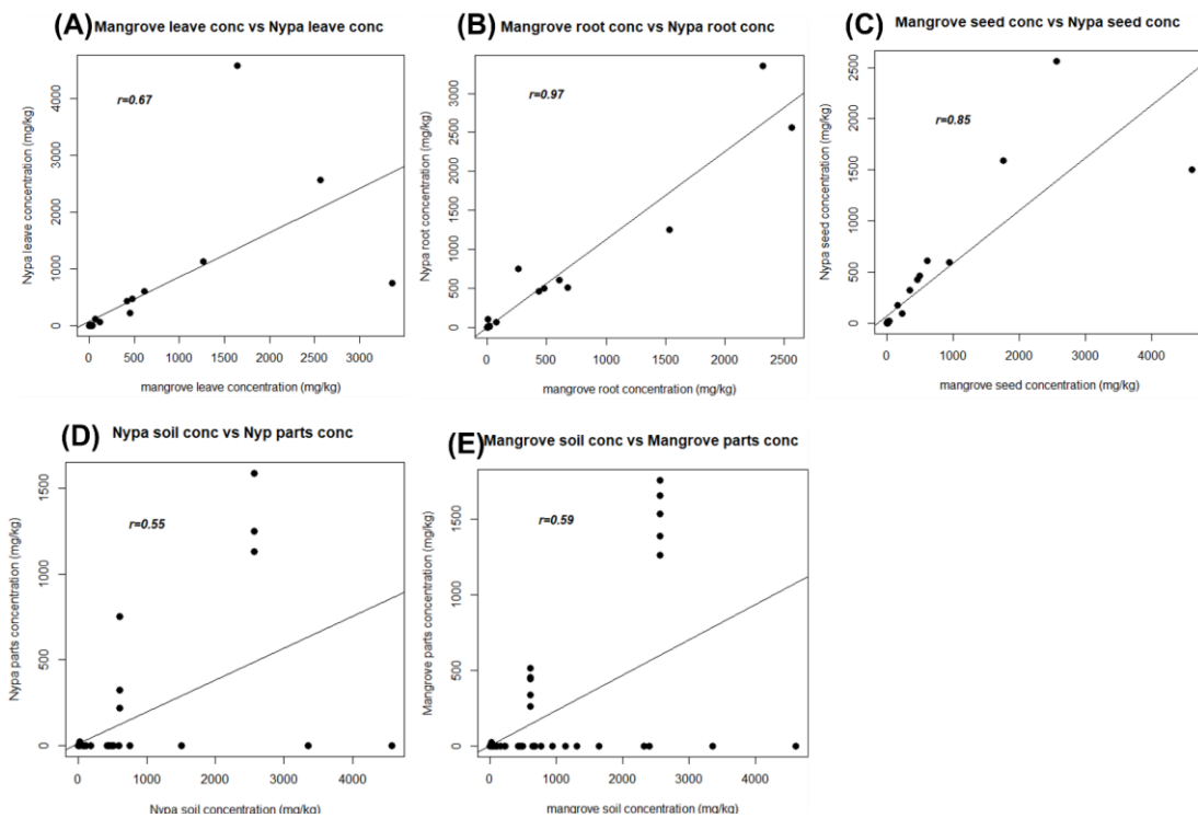
Fig. 7. Correlation of mangrove parts concentration versus nypa parts concentration for (A) leaf, (B) root, (C) seed, (D) nypa soil and (E) mangrove soil collected at Eagle Island, Niger Delta Nigeria
