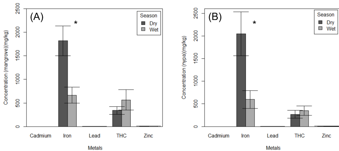
Fig. 8. Mean seasonal effect of THC and heavy metal (±SE) on (A) mangrove and (B) nypa palm treated soils collected from Eagle Island, Niger Delta, Nigeria
