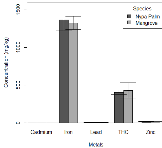
Fig. 3. Mean concentration of THC and heavy metals ( \pm SE) in mangrove and nypa palm treated soils collected from Eagle Island, Niger Delta, Nigeria
