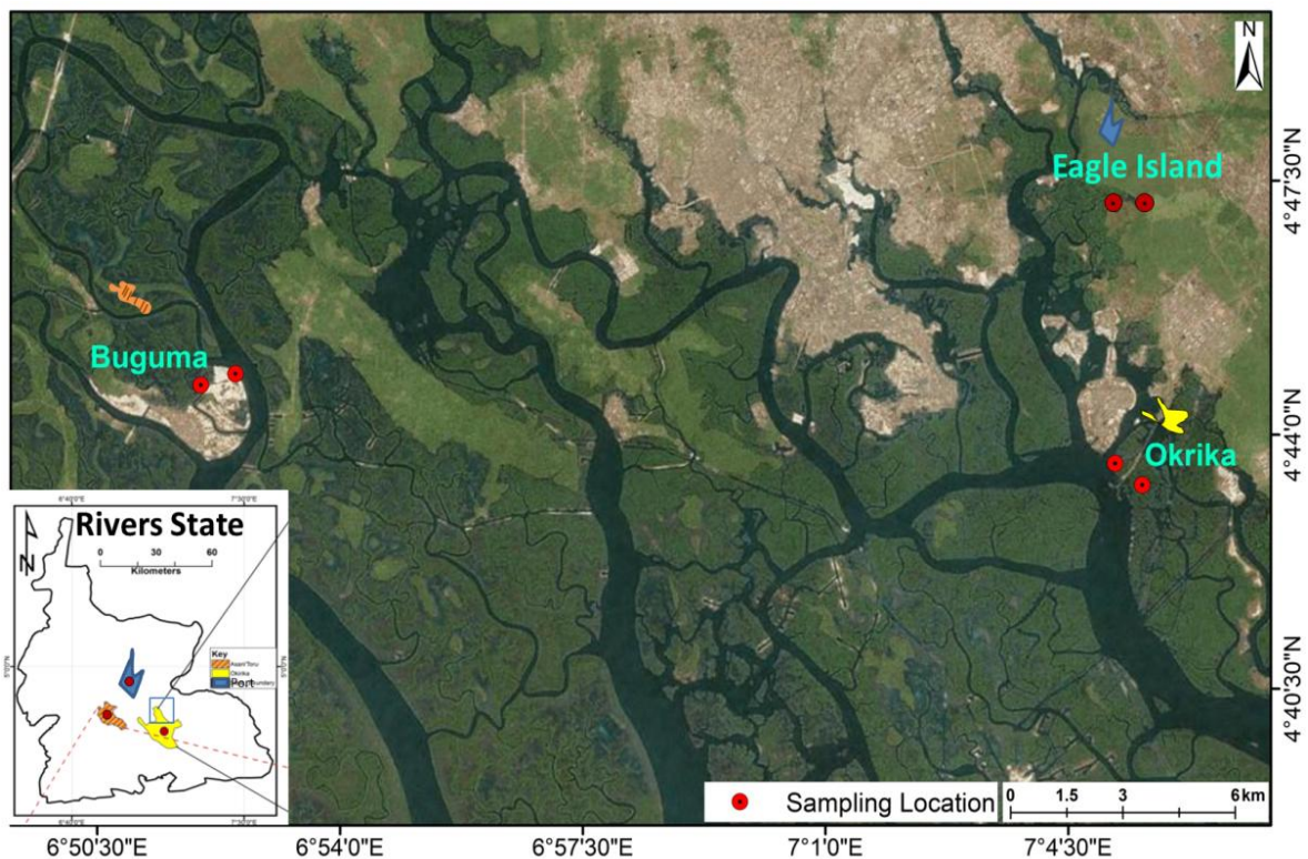
Fig. 1. Map of study area where mangrove and nypa parts and soil samples were collected at Eagle Island, Niger Delta, Nigeria
