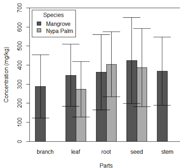
Fig. 4. Mean concentration of THC and heavy metal ( \pm SE) in mangrove and nypa palm parts collected from Eagle Island, Niger Delta, Nigeria
