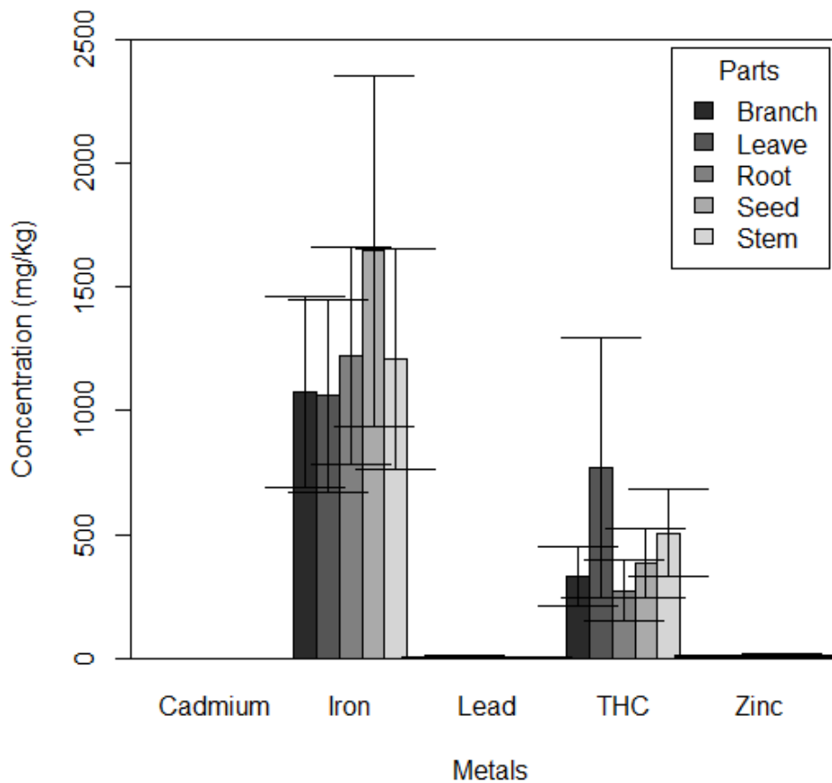
Fig. 7. Mean concentration of THC and heavy metals ( \pm SE) in mangrove part treated soils. Leaf treated soil have the lowest concentration of Fe whereas root treated soil have the lowest THC concentration
