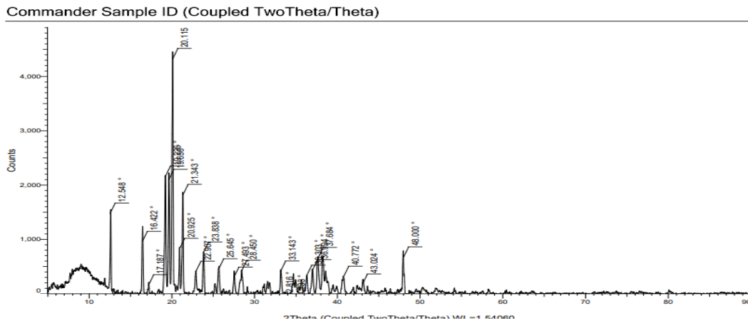
Fig. 4(A). X-RD analysis of WPC
