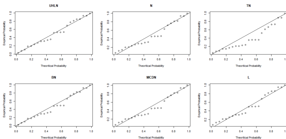
Fig. 2. Probability probability plot of the fitted distributions for dataset I
