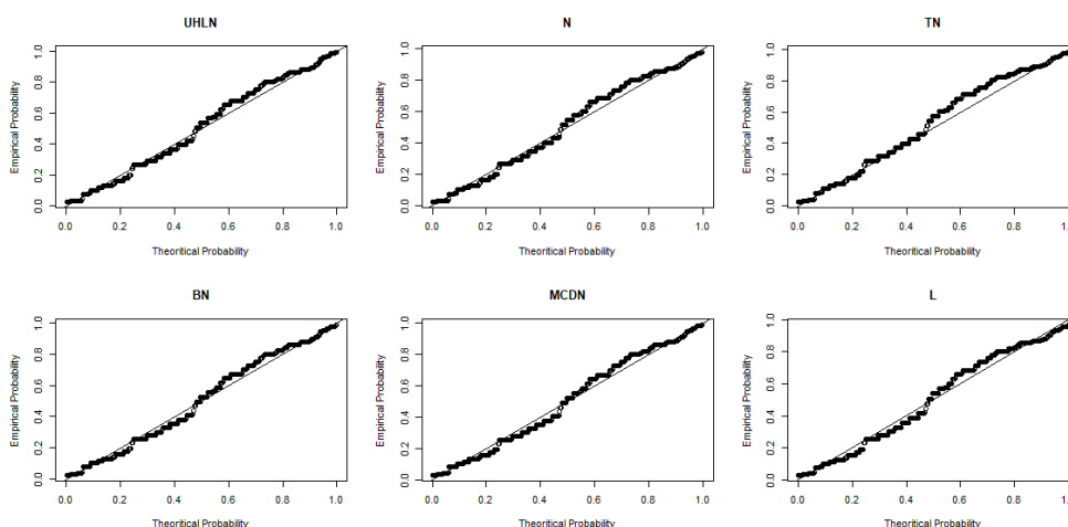
Fig. 4. Probability probability plot of the fitted distributions for dataset III
