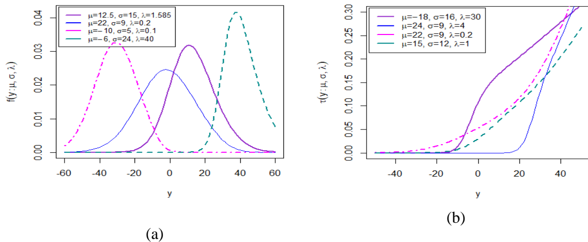
Fig. 1. (a) PDF and (b) Hazard plot of the UHLN distribution
