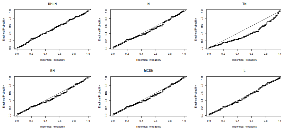
Fig. 3. Probability probability plot of the fitted distributions for dataset II
