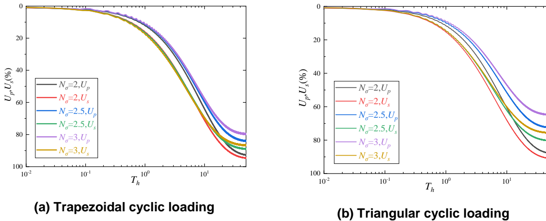
Fig. 8. Average degree of consolidation at different values of N_\sigma
