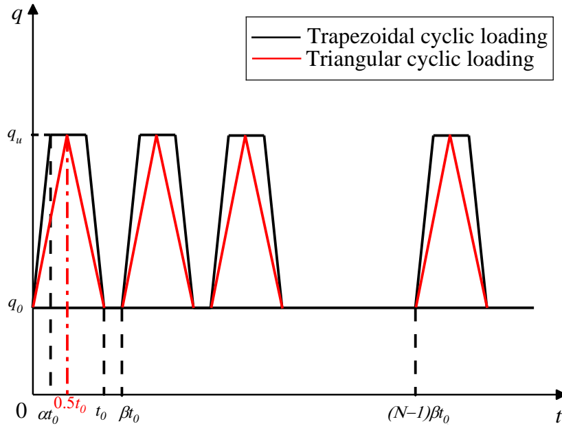
Fig. 3. Schematic diagram of Trapezoidal and Triangular cyclic loadings
