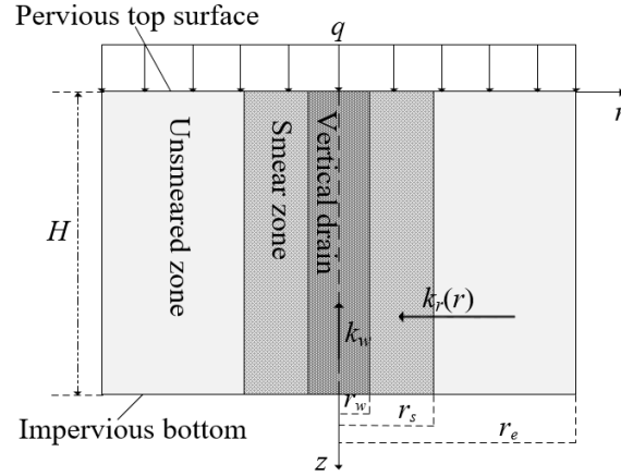
Fig. 1. Calculation model for vertical drain
